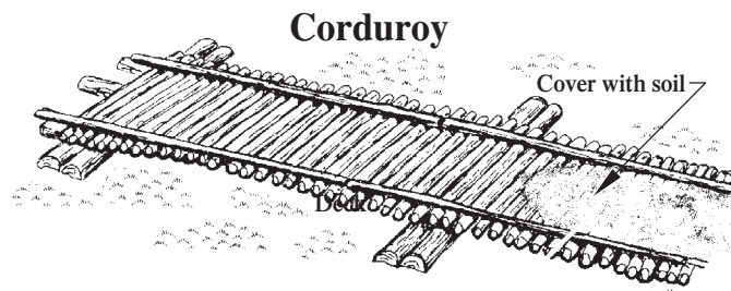
Figure 55—Corduoy should be considered a temporary fix until a more permanent structure can be installed.
